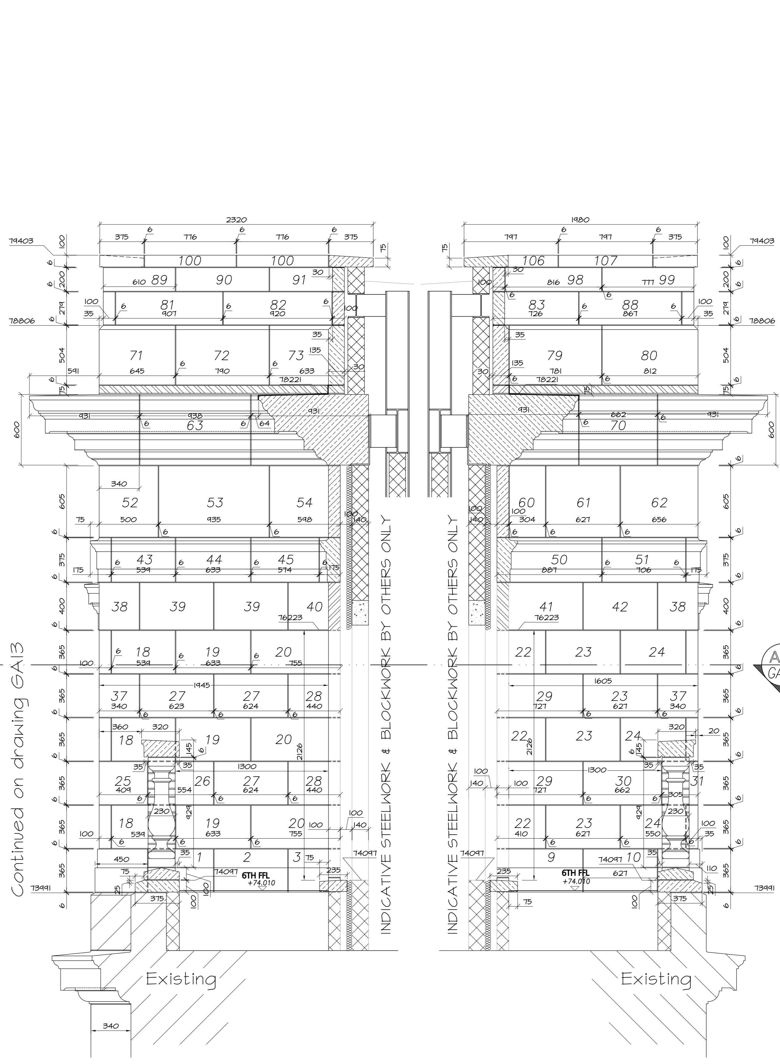
Section 1-1
